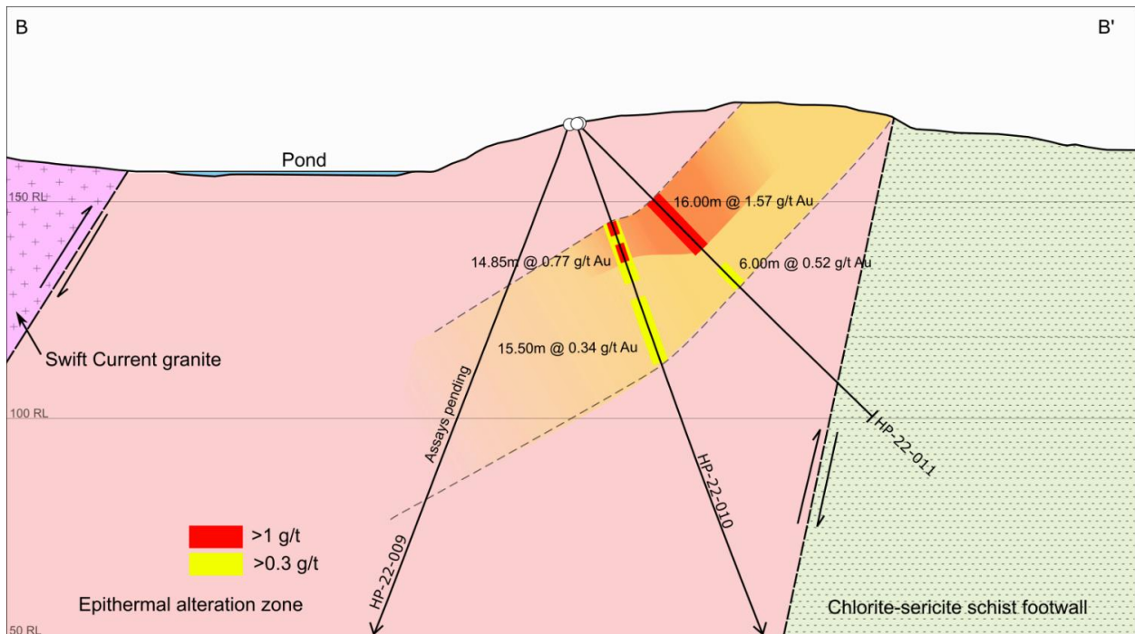
Figure 5: Schematic section through the Hickey's Pond system, section B-B' (see plan map). Assays for hole HP-22-009 are pending.
